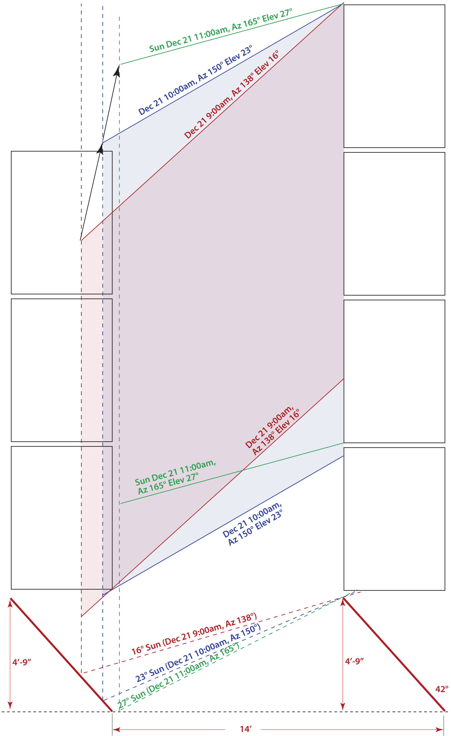
Solar Panel Spacing Details September 28, 2012 Scale: 1/2" = 1'
